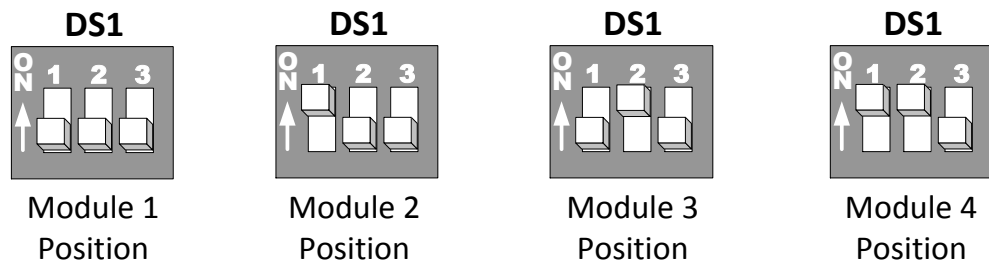
Illustration 4 - DIP Switch Module Position Settings
