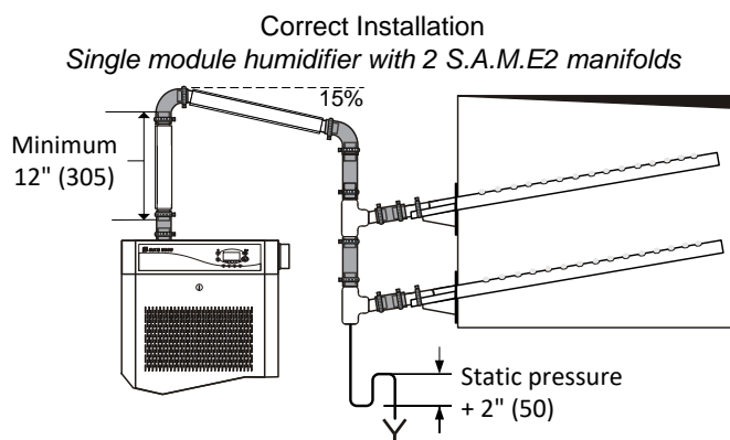
Steam distribution correct installation 2 - Fig. 15b (dimensions in bracket are in mm)
