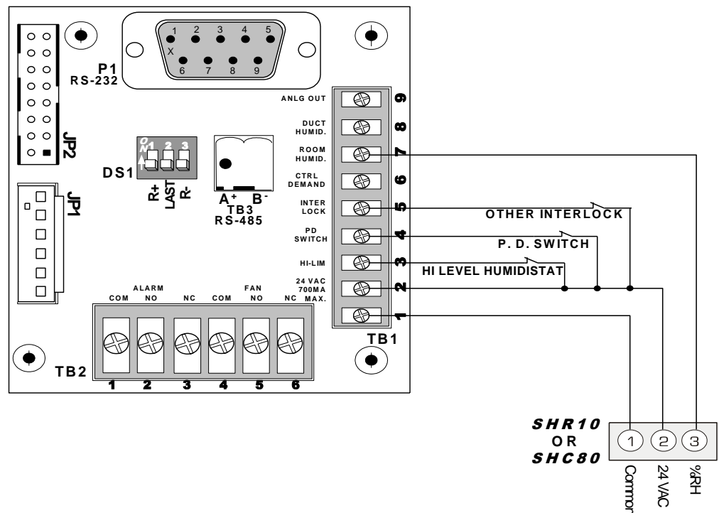
Humidity signal from humidity sensors - Fig. 45
