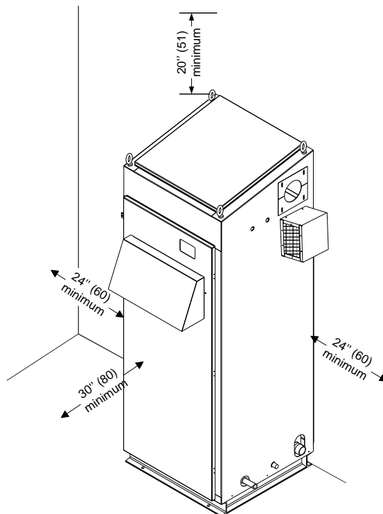
Weather proof enclosure clearance - Fig. 13 (dimensions in bracket are in mm)
