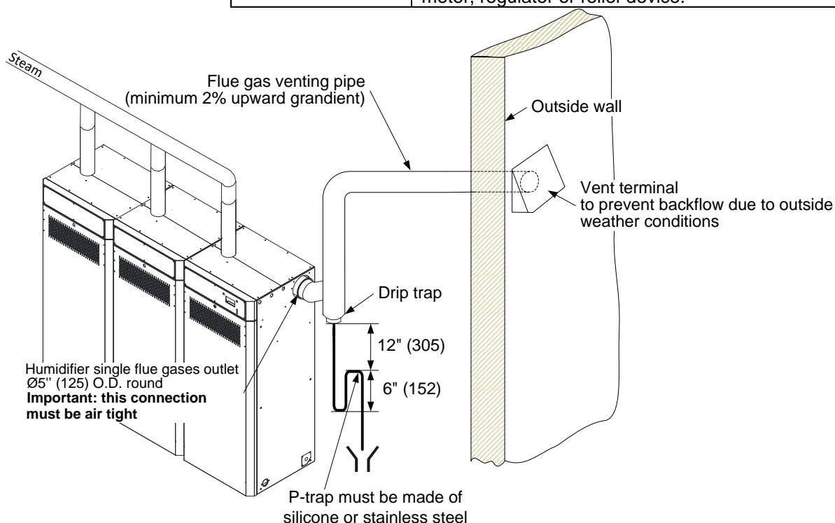
Typical flue gas installation, 3 modules - Fig. 40 (dimensions in bracket are in mm)
