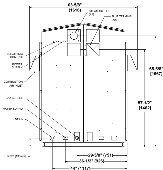
Weather proof enclosure Connection positions 4 modules - Fig. 8 (dimensions in bracket are in mm)
