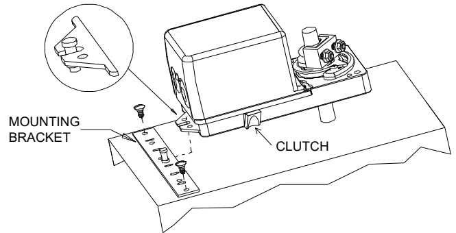
EVCB44N with a built-in 70 in. lb. Actuator
