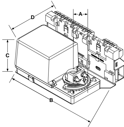
EVC with a separate 180 in. lb. Actuator
